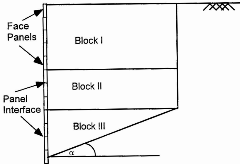
Fig. 5: Proposed Three-Block Model for Wall Deformation.
