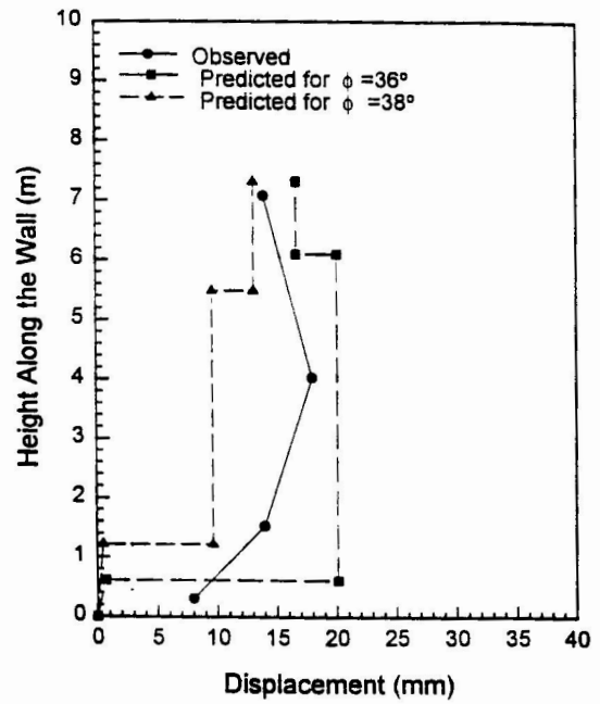
Fig. 6: Predicted and Computed Wall 1 Displacement in Event N.
