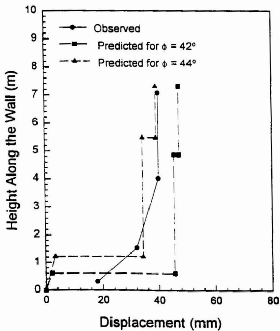
Fig. 7: Predicted and Computed Wall 5 Displacement in Event L.
